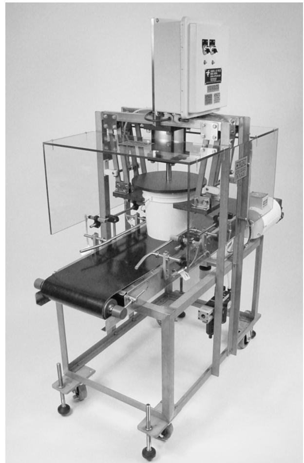
Shown with Optional Container Support Assembly
