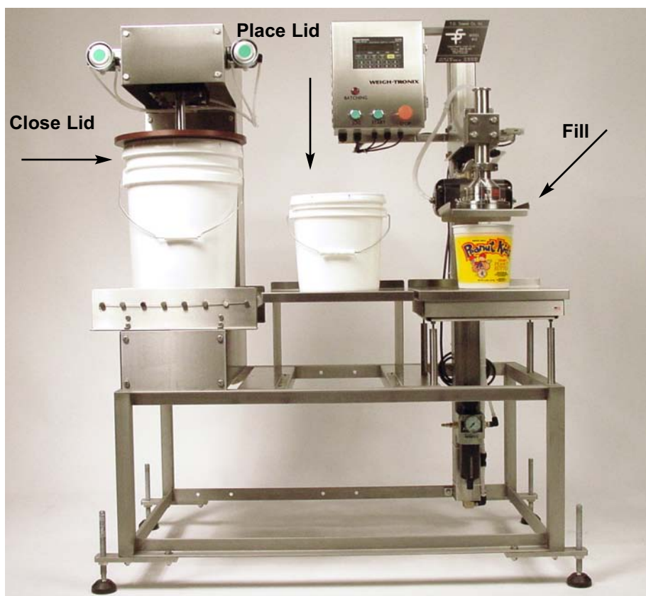
Shown with Left Hand Product Discharge and Optional Sawvel 119 Manual Lid Press
